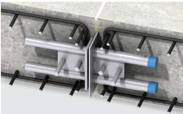
ANCON Shear Load Connector
