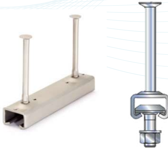
Jordahl Anchor Channel JTA K
